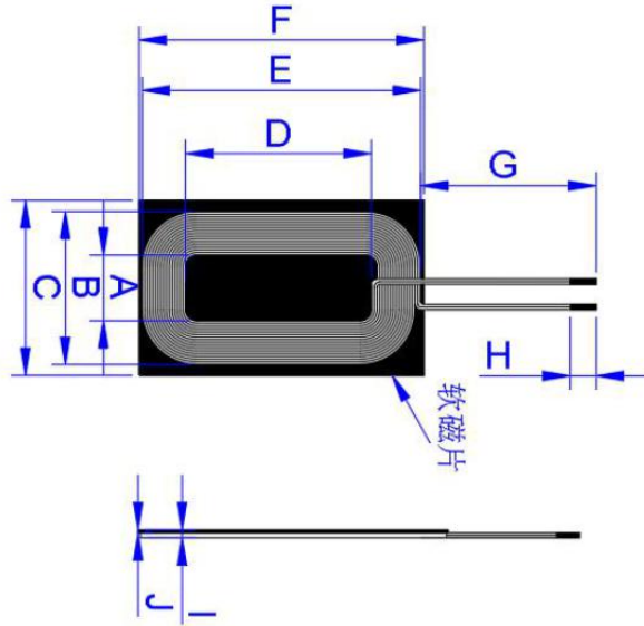
Figure 1. Physical dimensions of the product.
